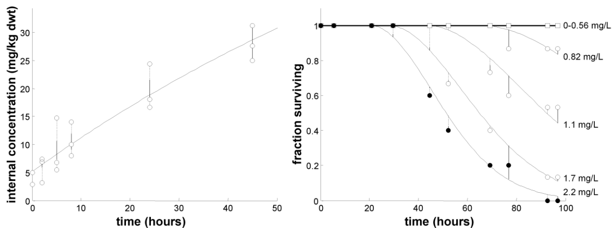
Figure 2. Simultaneous analysis of body residues (at 0.1 mg/L, left plot) and mortality with DEBtox for cadmium (0-2.2 mg/L, right plot) in Daphnia magna at 10 °C (no food). In the right plot, model lines indicate different exposure concentrations (squares are control, black dots the highest dose).
